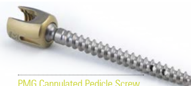
PMG Cannulated Pedicle Screw Polyaxial/Monoaxial Ø5.5- Ø8.5 mm Titanium
